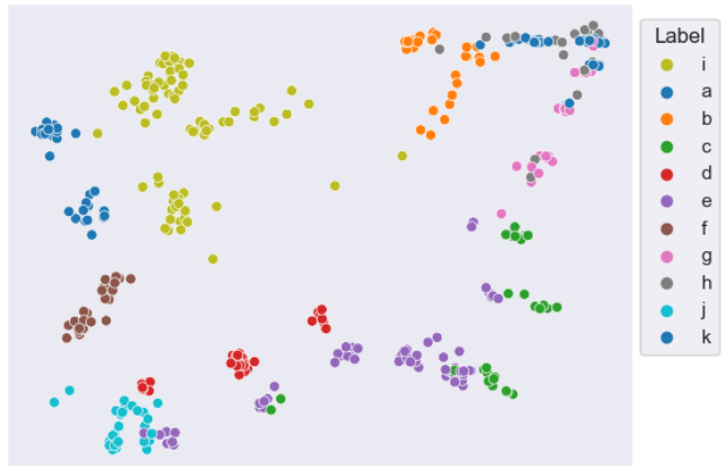
Fig. 6: Scatter plot showing syllables from the song of one Bengalese finch, embedded in a 2-D space using a convolutional encoder trained using the Parametric UMAP algorithm. Each marker is a point produced from a spectrograms of a single syllable rendition, mapped down to the 2-D space, from 40 seconds of training data. Colors indicate the label applied to each syllable by an expert human when annotating the spectrograms with a GUI.
